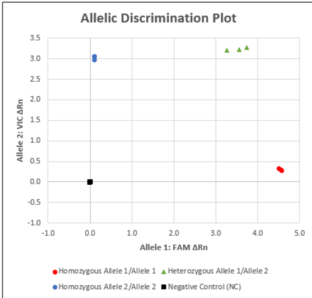
Allelic discrimination plot
